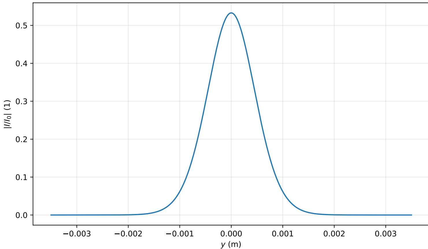
Intensity profile I(x=0, y, z=2.468)/I_0 , P_{in}=0.3P_{cr} , artificial time
